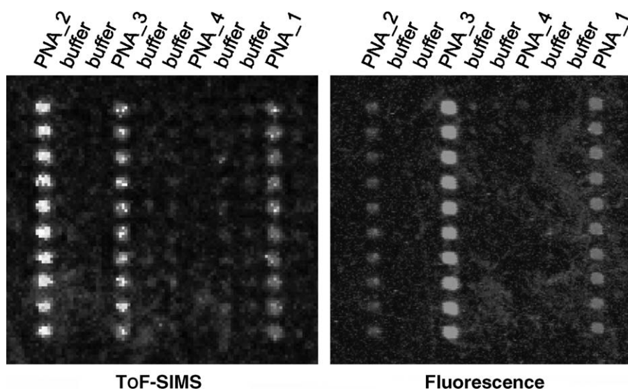
Fig. 5. Comparison of ToF-SIMS and fluorescence detection. Following molecules were spotted in columns of 10 replicates from left to right onto maleimide slides: PNA_2, buffer, buffer, PNA_3, buffer, buffer, PNA_4, buffer, buffer, PNA_1. Hybridisation of the slide for ToF-SIMS detection was done with three unlabelled DNA oligomers (DNA_1, DNA_2 and DNA_3) while for the fluorescence detection corresponding Cy3- and Cy5-labelled oligonucleotides were used. The results for \text{PO}_3^- and fluorescence intensities are shown.
