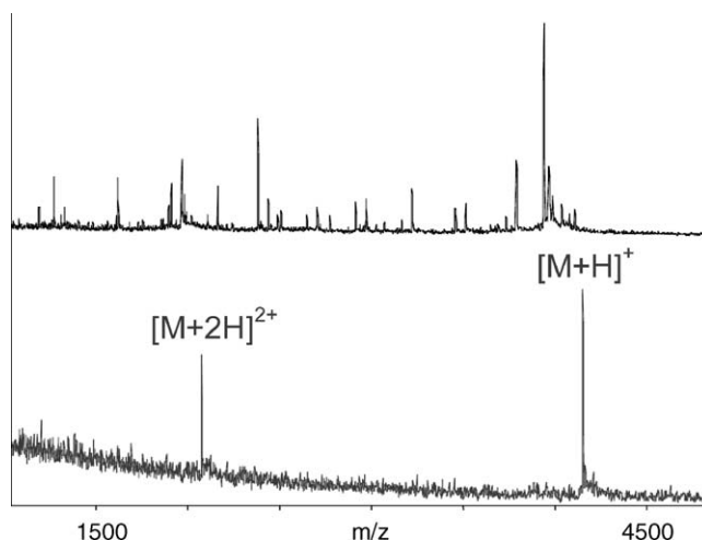
Fig. 4. Efficiency of the on-chip purification. MALDI-ToF spectra of an example for a crude PNA (top) and the same PNA, which was spotted, washed and cleaved from the chip surface (bottom). The mass shift of the PNA molecule is due to the cleavable linker that was used on the surface.
