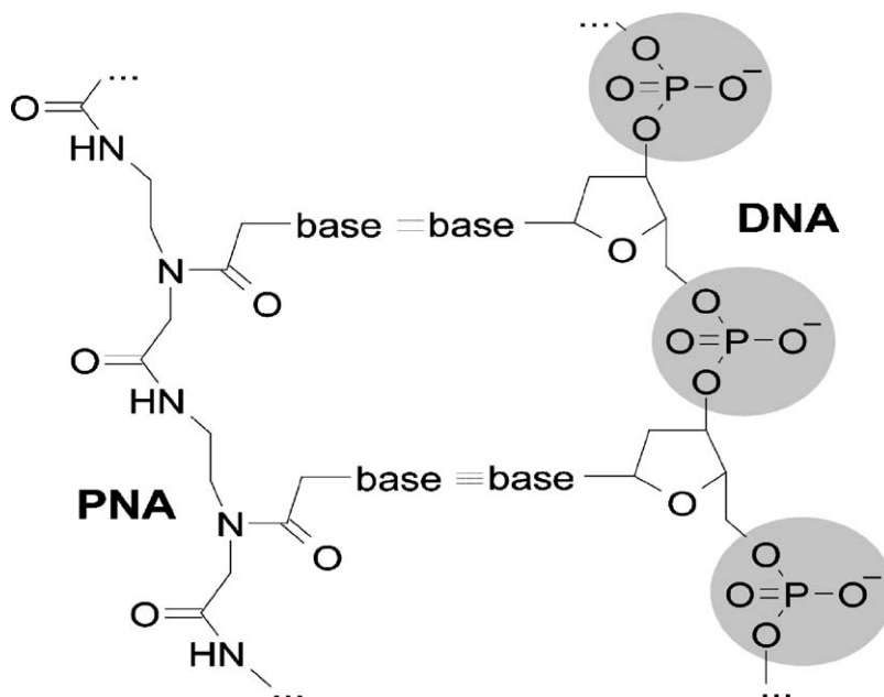
Fig. 1. PNA:DNA duplex with characteristic backbones.
