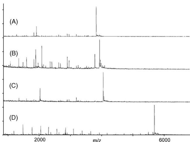
Fig. 2. MALDI-ToF-MS spectra of PNAs synthesised in microtiter plates. Following PNAs are shown: cysteine-Li-TTGAATCGCTCGA-Li-CONH 2 (A), Li-TTGAATCGCTCGA-Li-CONH 2 (B), biotin-Li-TTGAATCGCTCGA-Li-CONH 2 (C) and Li-Li-CCATACAAATTTTCAGGATTT (D).
