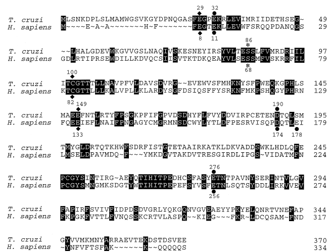
Figure 10 Comparison of the amino acid sequences of the T. cruzi and the human AdoMetDC proteins
