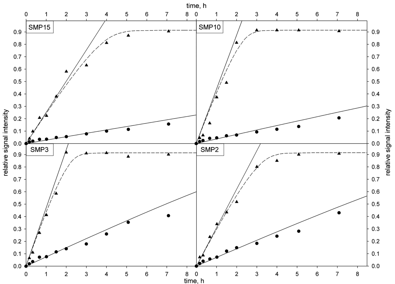
FIG. 2. Development of the relative signal intensity over time for the anti-IFNG spots of different radius: SMP15 (272- \mu\text{m} radius; upper left), SMP10 (190 \mu\text{m} ; upper right), SMP3 (86 \mu\text{m} ; bottom left), and SMP2 (45 \mu\text{m} ; bottom right) under stirring ( \blacktriangle ) and non-stirring ( \bullet ) conditions. The progression curves were fitted to Equation 1 (---) as well as simulated using Equation 3 (—).
