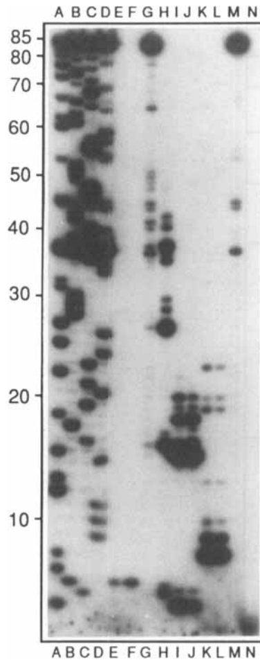
Figure 3. Autoradiogram of a gel from E. coli DNA polymerase I-catalyzed incorporation of BrdITP by template:primer. Lanes A-D: sequencing lanes for products ending with A, G, C and T, respectively. Incubations were done for 40 min with the additions indicated. Lanes E,F: 20 \mu M dGTP, dCTP and dTTP, plus 180 \mu M BrdITP (E) or no analog (F). Lanes G,H: 20 \mu M dATP, dCTP and dTTP, plus 180 \mu M BrdITP (G) or no analog (H). Lanes I,J: 20 \mu M dGTP, dATP and dTTP, plus 180 \mu M BrdITP (I) or no analog (J). Lanes K,L: 20 \mu M dGTP, dATP and dCTP, plus 180 \mu M BrdITP (K) or no analog (L). Lanes M,N: 20 \mu M dATP, dCTP, and dTTP, and 180 \mu M dGTP, with pol I (M) or without pol I (N).
